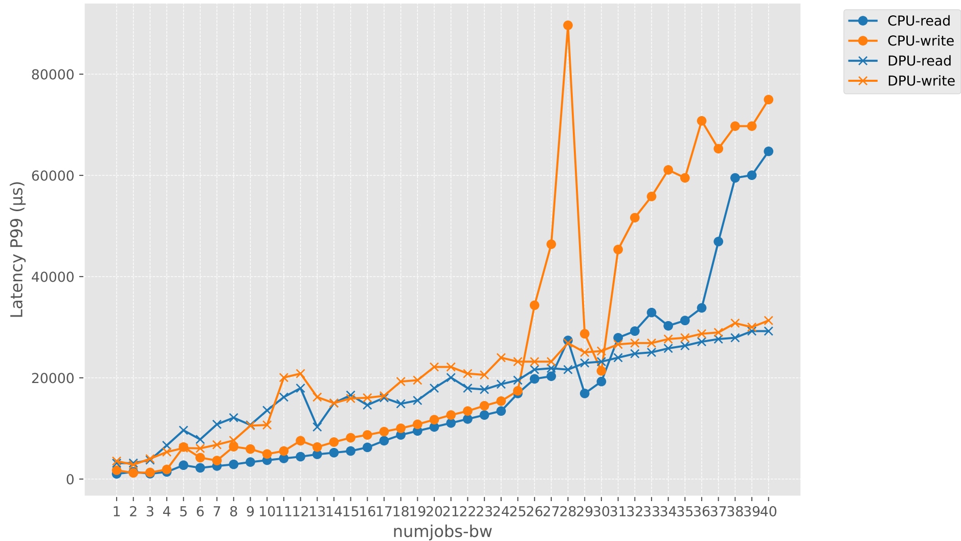
Latency P99 vs numjobs-bw (CPU vs DPU)
